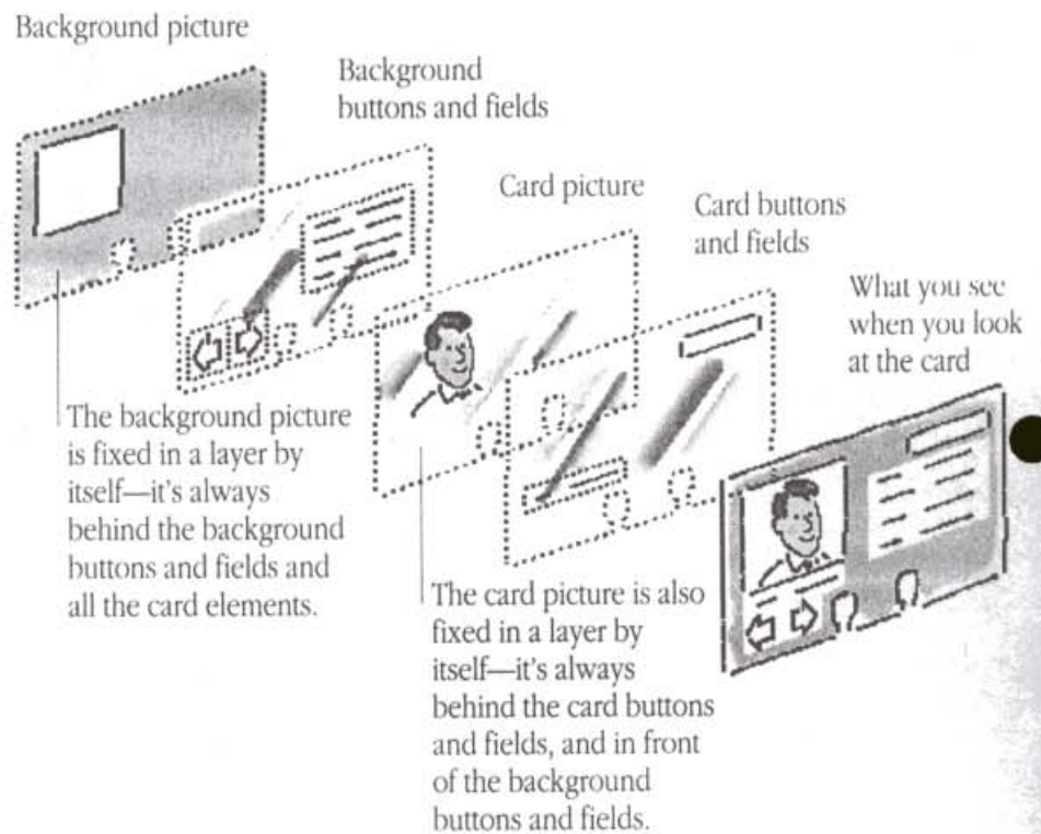
Figure 6-44 HyperCard's layers
