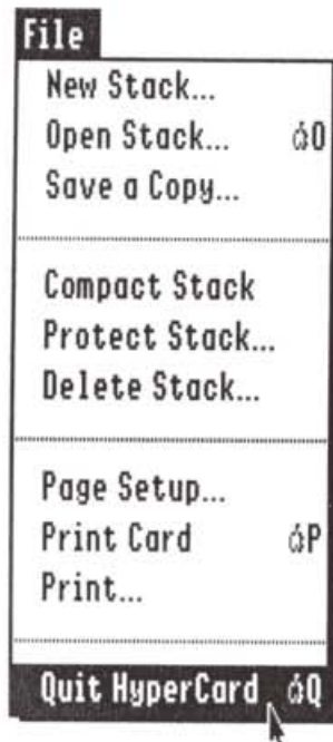
Figure 1-41 Quitting HyperCard
