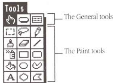
Figure 2-10 HyperCard's tools
