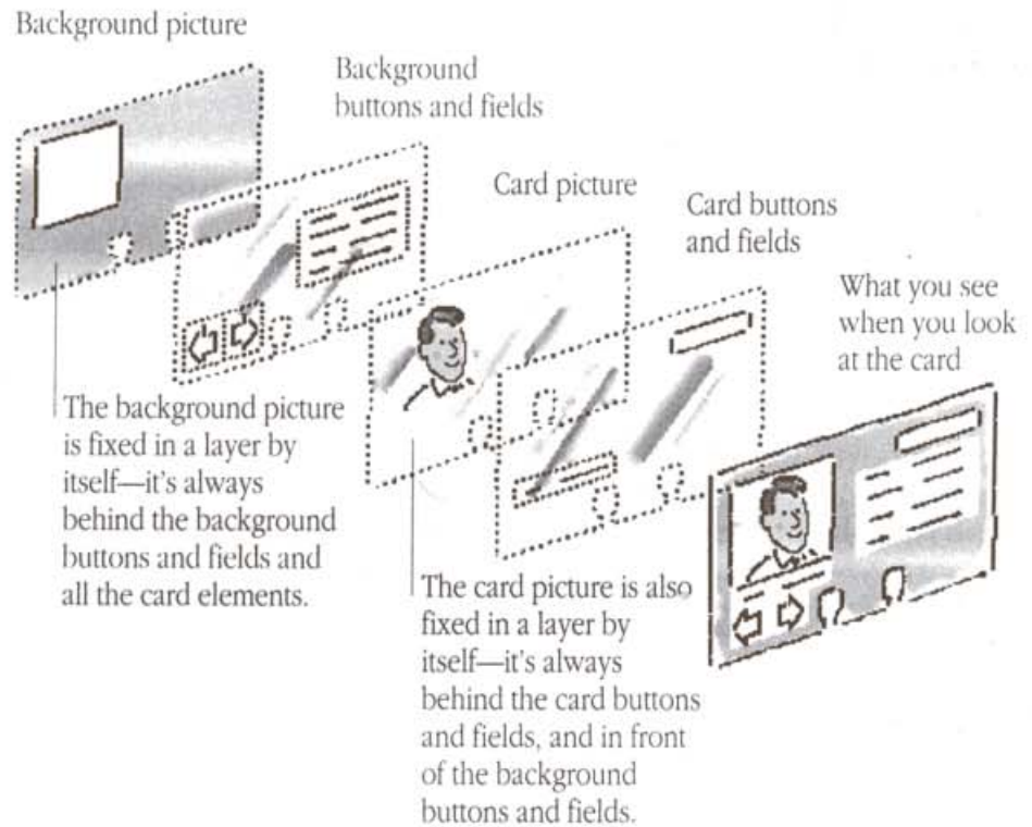
Figure 5-24 HyperCard's layers
