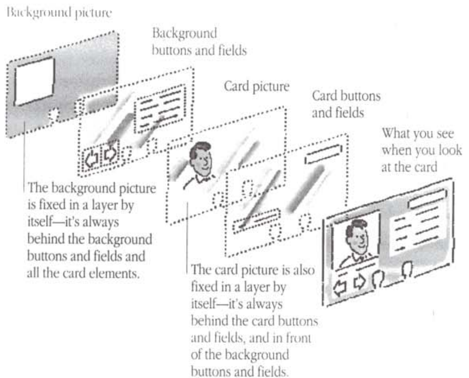
Figure 4-38 HyperCard's layers
