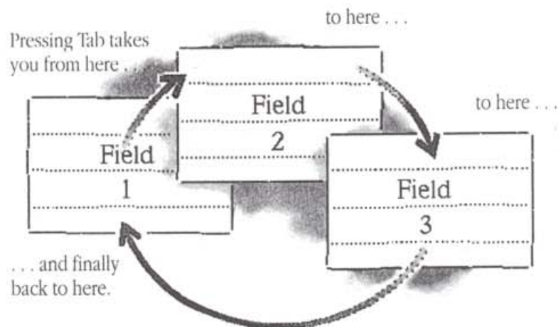
Figure 5-7 Tabbing order
