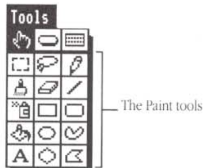
Figure 6-1 HyperCard's tools
