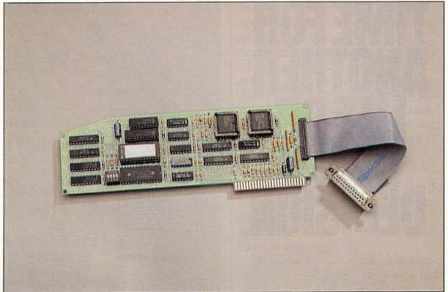
Apple II High-Speed SCSI Card
