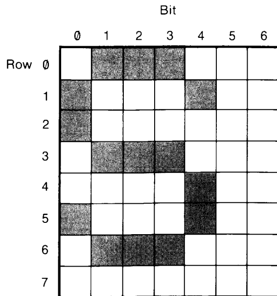
Format of a Character Cell
