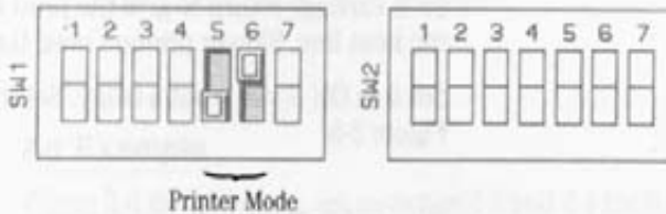
Figure 2-3. Printer Mode Setting
