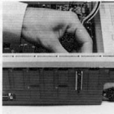
Figure 1-4. Hold Connector and Nut Plate up to Back Panel
