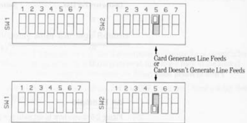
Figure 2-7. Line Feed Settings
