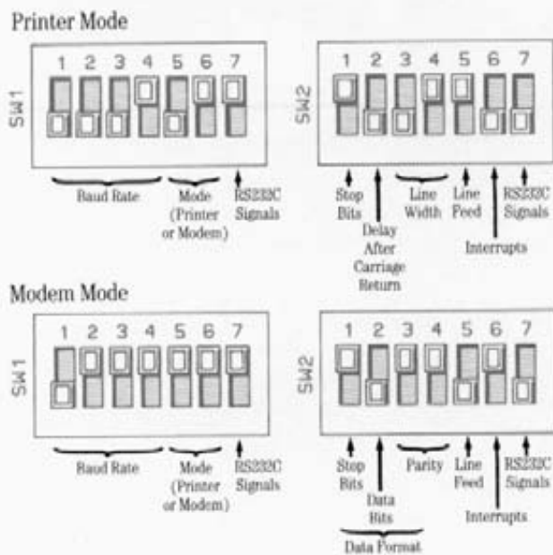
Figure 2-1. What the Switches Do
